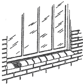
Sill Brick SS-H
