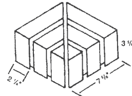
2-Piece Corner SS-OC Also match SS-OGH
