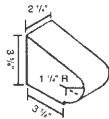
Sill Brick SS-H
