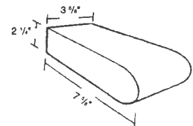
Coping SS-C Also used as pool coping
