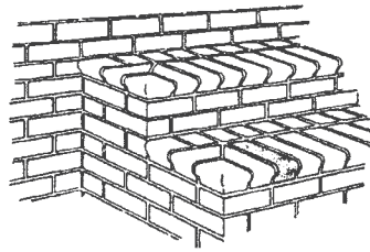
Step Tread SS-OGH
