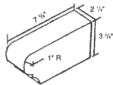
Step Tread SS-OGH
